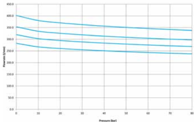
Flowrate GR55 SM @ 2750 RPM - 68 cSt
